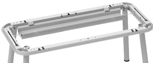
Metal cable duct, rear or centre mounting
